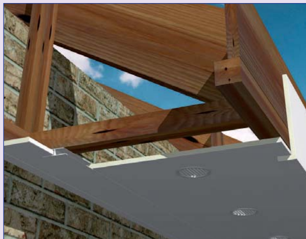
9mm Square Edge Fascia – Multi-purpose board as a Soffit vented with disc vents
